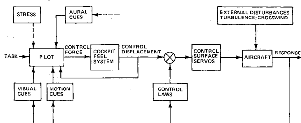
Fig. 1 Pilot-vehicle dynamic system.
