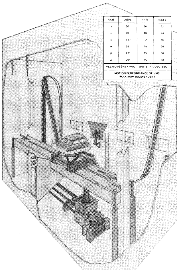
Fig. 7 Modern 6-DOF motion-based research ground simulator (NASA Ames VMS).
