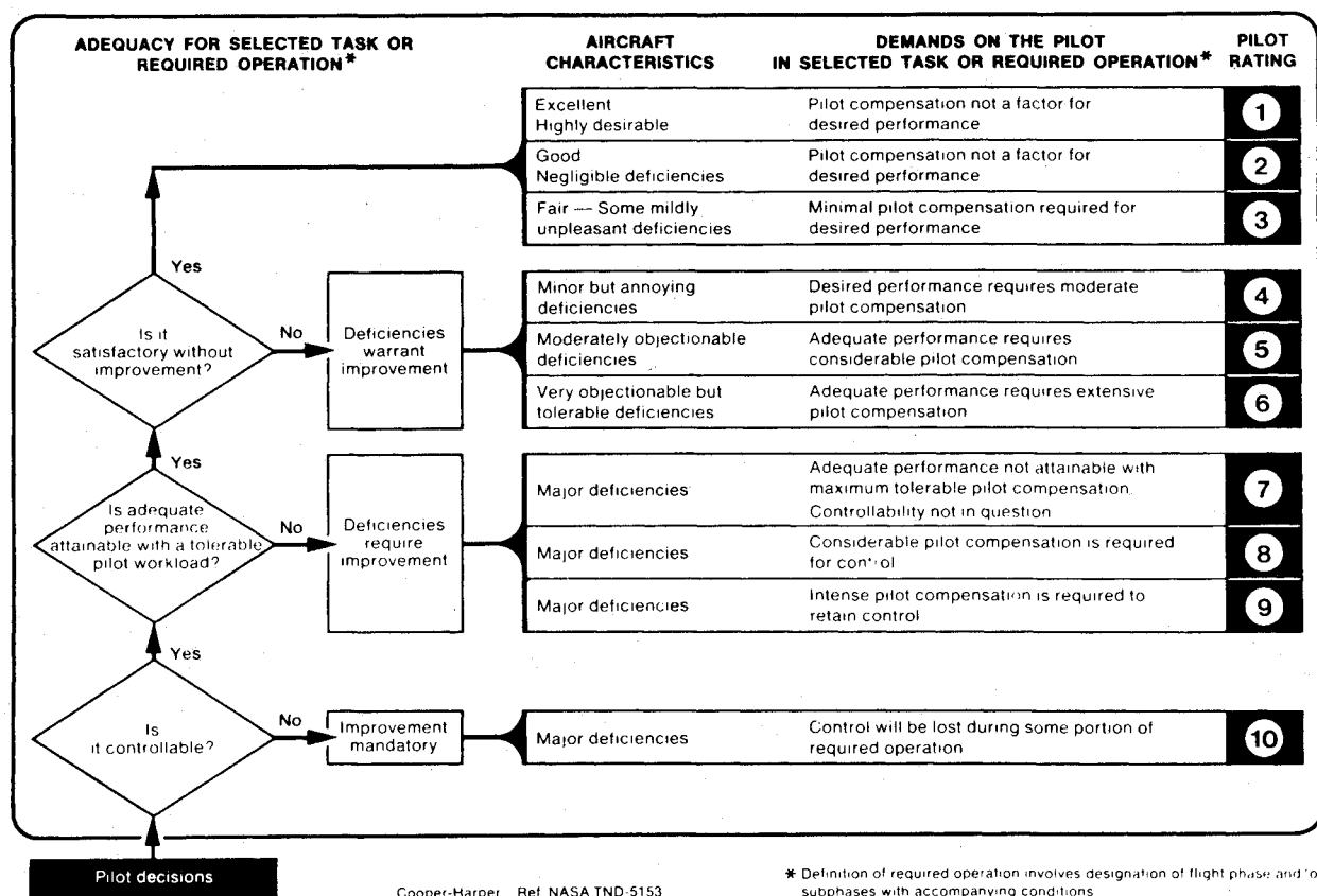
Fig. 8 Cooper-Harper handling qualities rating scale.
